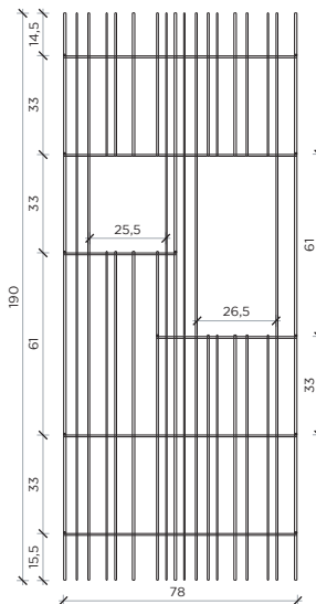
FRONTE | FRONT
