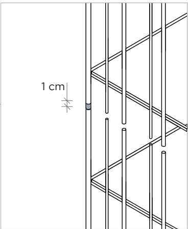
VERTICAL JOINTS
