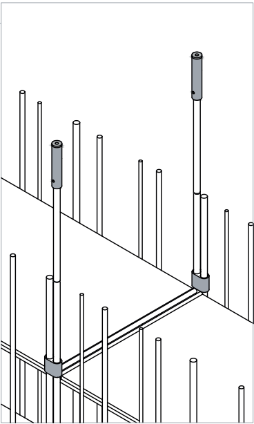
HORIZONTAL JOINTS
